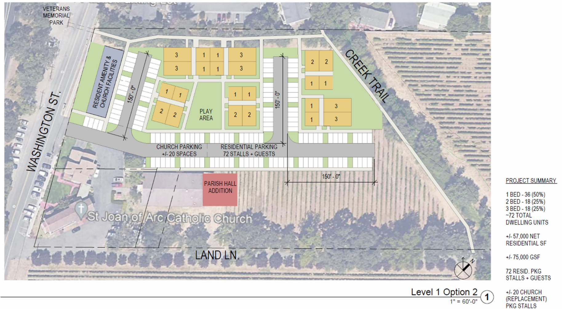
Figure E-4: Site 2 – Conceptual Site Plan 2
